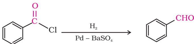
Benzoyl chloride
