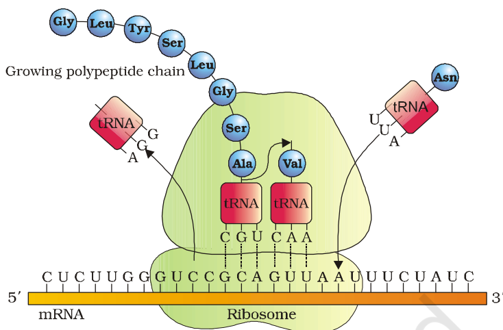
Figure 5.13 Translation
