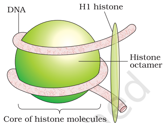
Figure 5.4a Nucleosome
