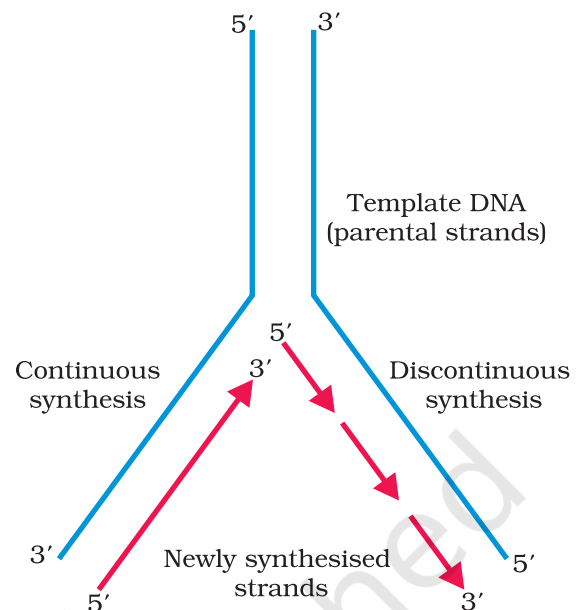
Figure 5.8 Replicating Fork
